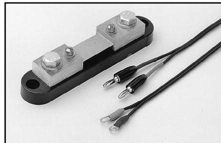
Model 1651 50 Ampere Shunt: External 0.001Ω ± 1%, 4-terminal shunt; extends current measuring capability of Keithley DMMs to 50A.
